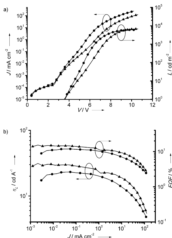
Figure 4. The current density-voltage-luminance ( J - V - L ) characteristics (a) and luminous efficiency ( \eta_L ) and EQE as a function of current density ( J ) (b) for the nondoped B-G2 (▲) and optimized doped device of H2:B-G0 (20 wt%; ●).
